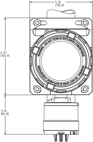
SST HOUSING SHOWN
