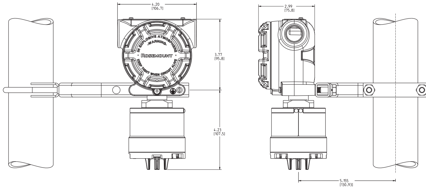
B4 BRACKET MOUNTING
